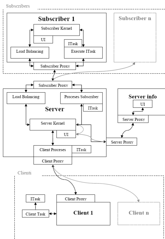
Fig.3. System modules interactions
